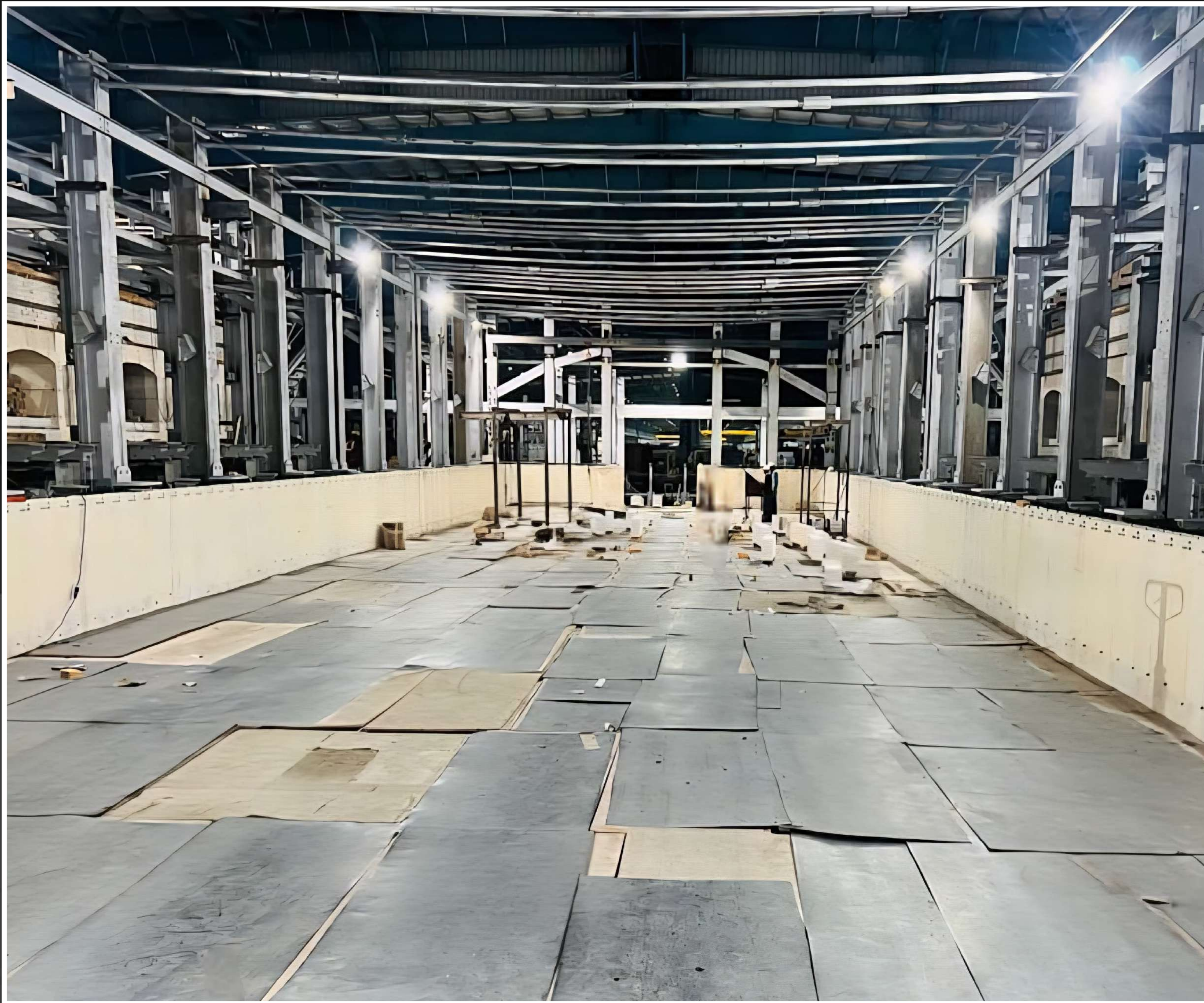
Erection of Refractories – Melting Tank & Refiner
